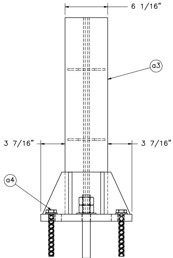
Back View
